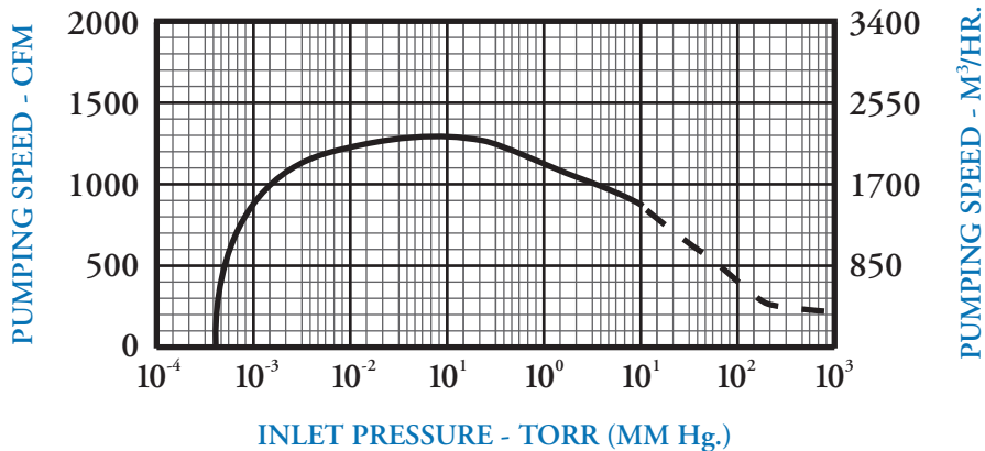
Curve Reflects Speed with 300 CFM Backing Pump
